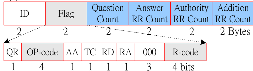
(b) DNS Header
