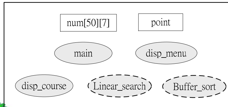
Ex4_5.java (Ex4_5.class)
